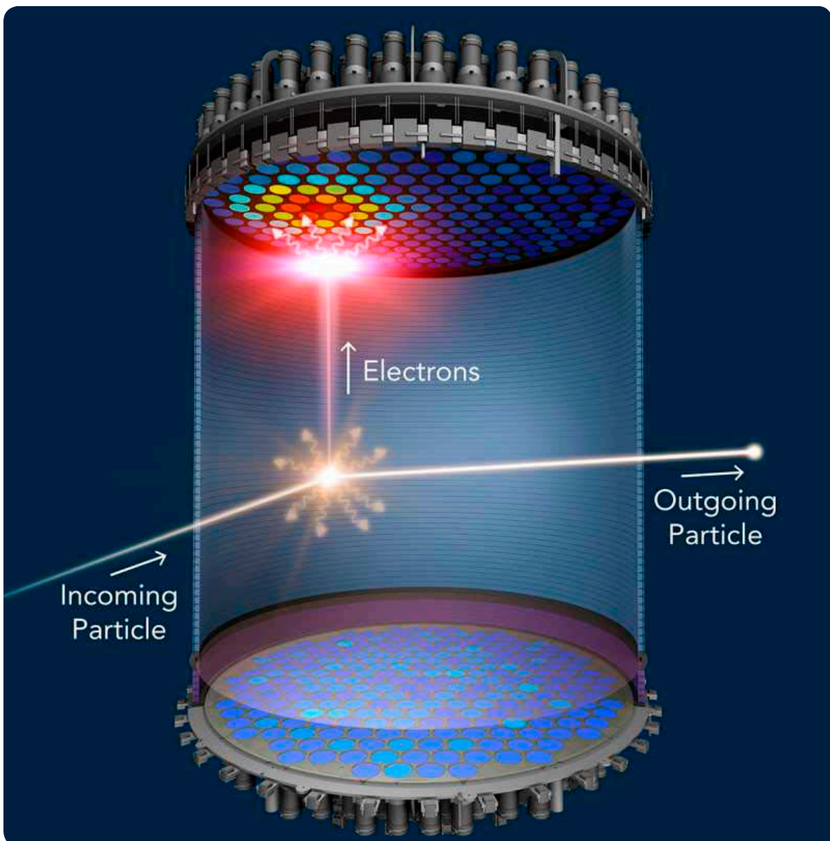
Dark matter detection principle
