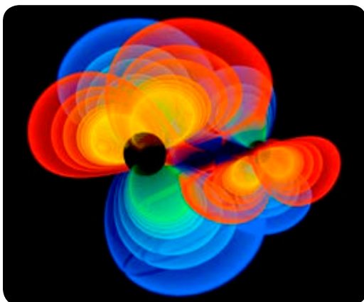
A simulation of black holes merging - first direct observation of gravitational waves (Credit: AEI/ITP/ZIB)
