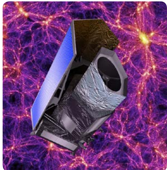
An artist's concept of the Euclid dark energy telescope in space (Credit: ESA)
