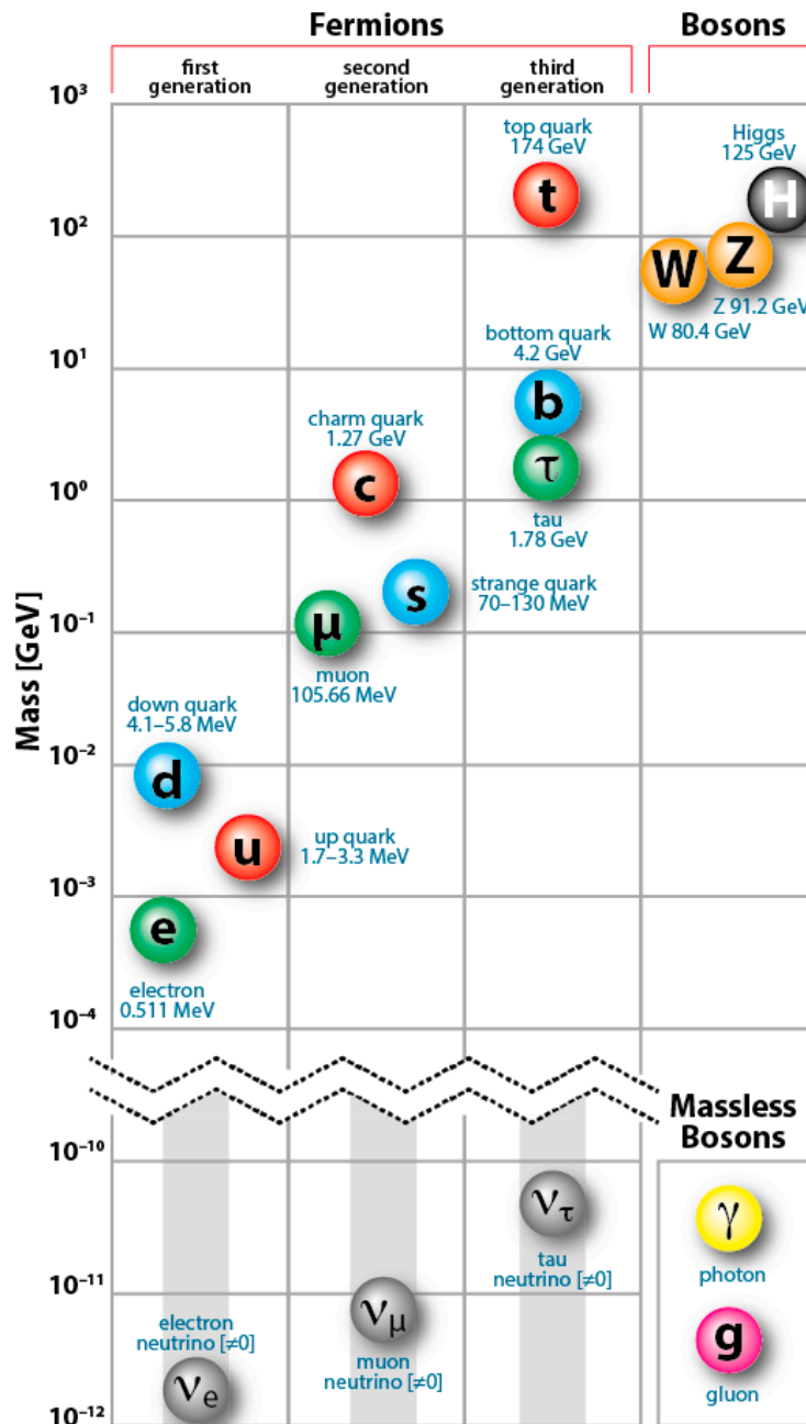
Standard model particle mass spectrum
