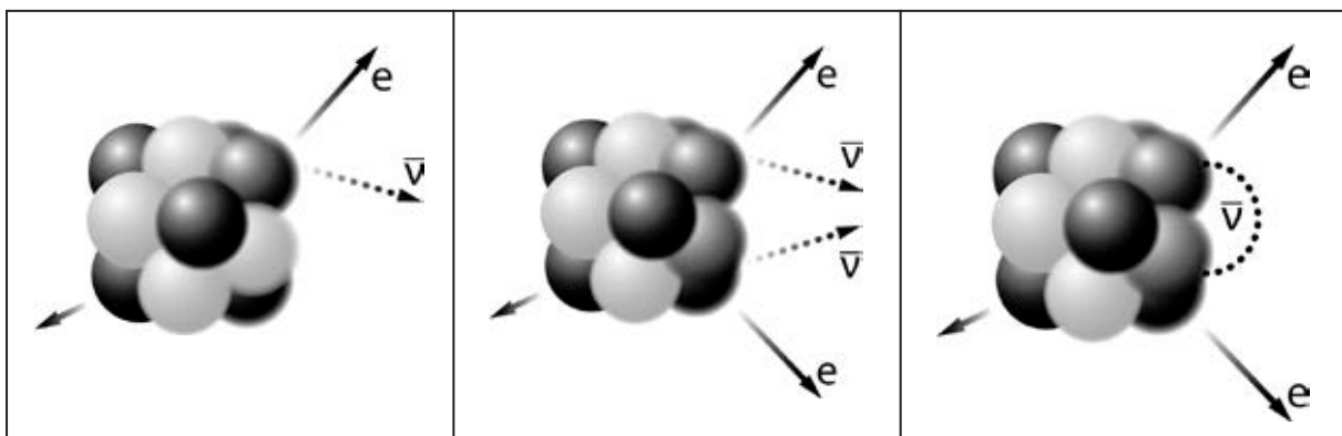
beta decay – e\nu
