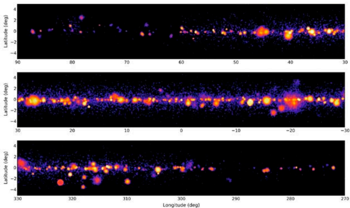
Identified sources of high-energy photon radiation in the plane of our Milky Way galaxy.
